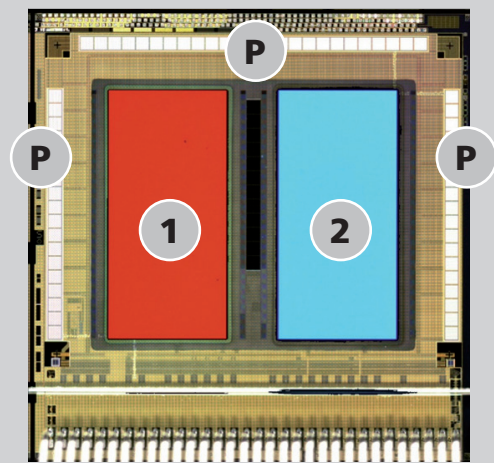
1 rote OLED 2 blaue OLED P Photodioden
